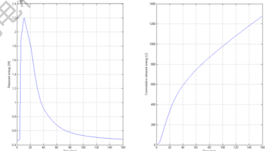
Figure 3: Total energy emitted by muzzle flash
