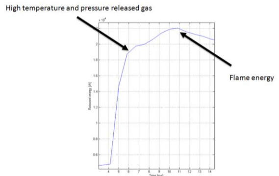
Figure 4: Total energy emitted (zoom on energy ramp-up)
